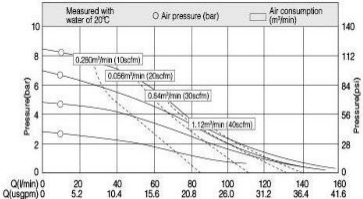
Performance curve
